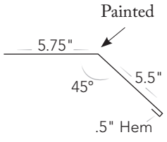
13 Gambrel Flashing
