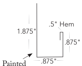
14 J-Channel
