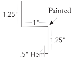
18 Wainscoat Trim not illustrated
