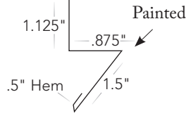
19 Rat Guard
