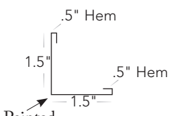
9 1.5" Angle not illustrated
