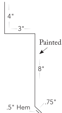
27 Square Door Track Cover
