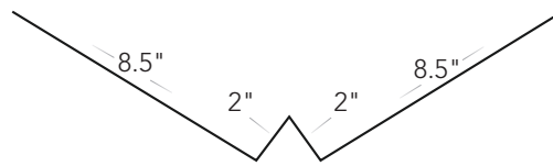
Valley #R-WV
