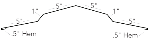
Ridge Cap #R-RC
