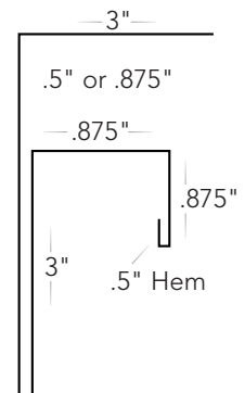
F-J Trim #T-FJ
