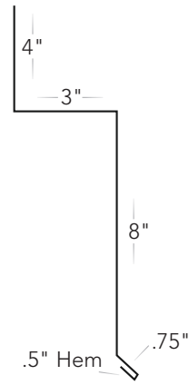
Square Door Track Cover #T-SDT
