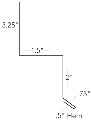
Wainscoat #R-WT
