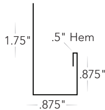
J-Channel #T-JC
