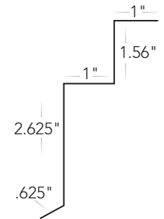
Z- Rake Cleat #S-ZRC
