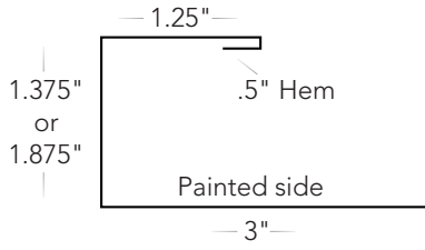
C-Channel #S-CC
