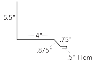
Sidewall #T-SW
