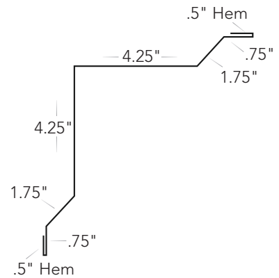
Inside Corner #R-IC
