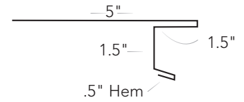
Extended Rake #S-ER
