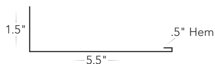
5.5" Angle #T-5.5A
