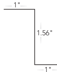
Z-Bar
