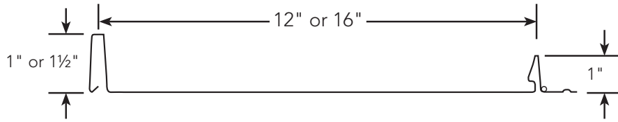
Screw Flange Panel
