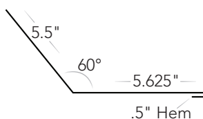
Endwall/Transition #T-EW
