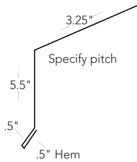
Eave #R-ET
