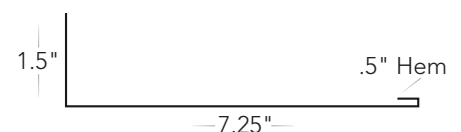
7.5" Angle #T-7.5A
