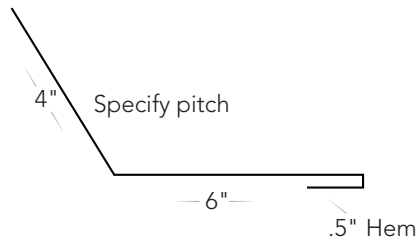
Endwall/Transition #R-EW
