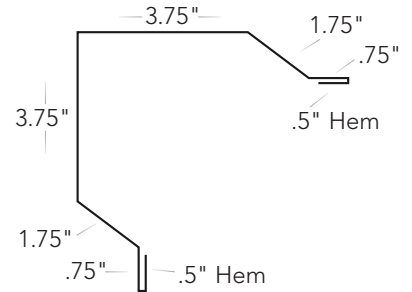
Outside Corner #R-OC
