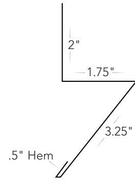
Rat Guard #R-RG
