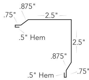
Narrow Outside Corner #T-OCN
