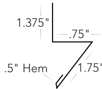
Rat Guard #T-RG
