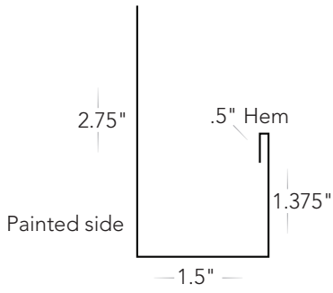
J-Channel #R-JC
