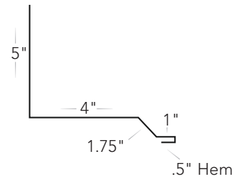
Sidewall #R-SW
