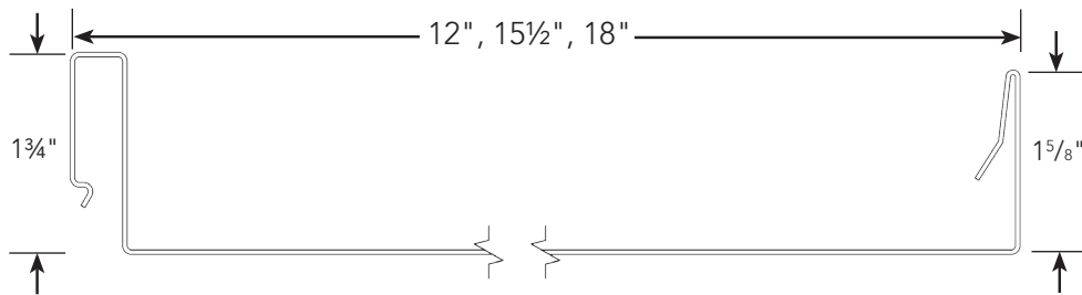
Clip Panel
