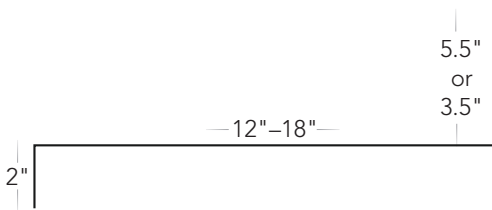
Soffit Trim #T-ST
