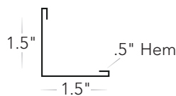
1.5" Angle #T-1.15A
