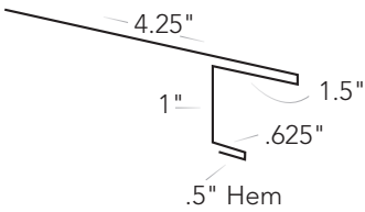
Extended Eave #S-EE
