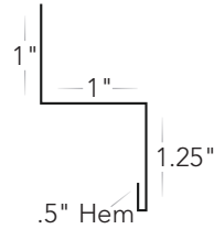
Wainscoat Trim #T-WT
