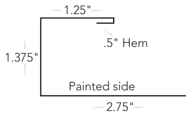
C-Channel #R-CC
