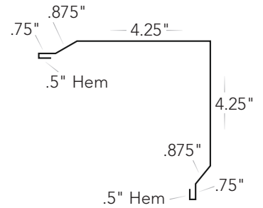
Wide Outside Corner #T-OCW
