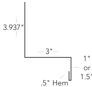
Sidewall #S-SW
