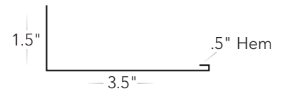
3.5" Angle #T-3.5A
